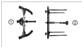
Motorcycle adaptor of wheel balancer
